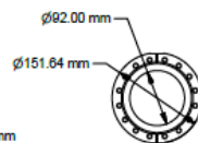
SECTION E-E SCALE 25
