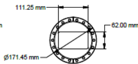
SECTION C-C SCALE 25
