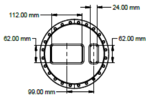
SECTION B-B SCALE 25
