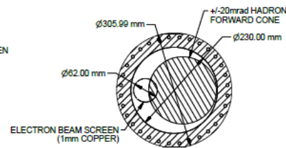
SECTION G-G SCALE 25
