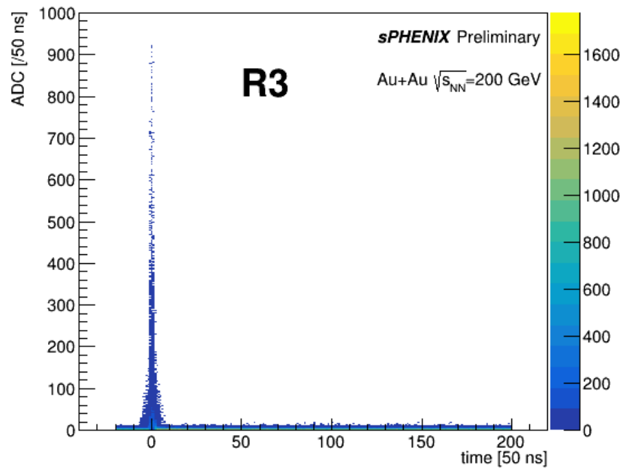
ADC vs Time Bins (Max Pad)
