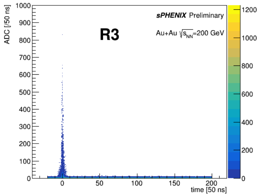
ADC vs Time Bins (Neighboring Pads)
