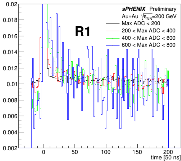
ADC vs Time Bins (Neighboring Pads)
