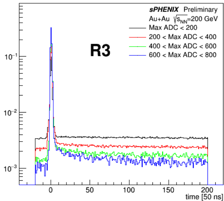
ADC vs Time Bins (Max Pad)
