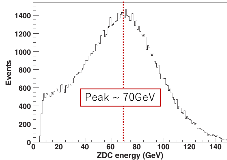
FIG. 10. The energy distribution measured with the ZDC after the neutron identification and the acceptance cut ( r < 2 cm, corresponds to p_T < 0.11 \cdot x_F GeV/c).
