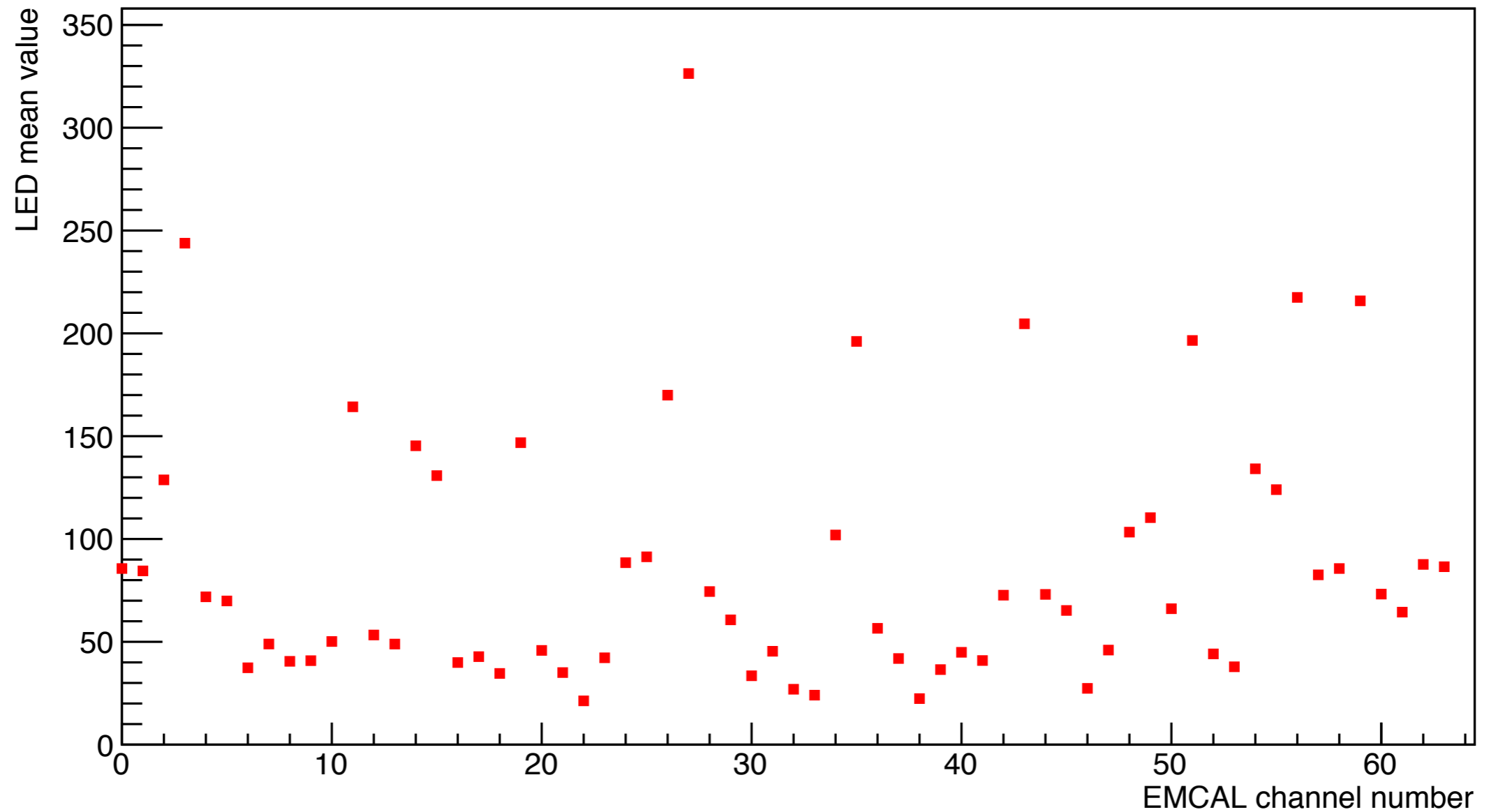
LED mean value vs. channel number
