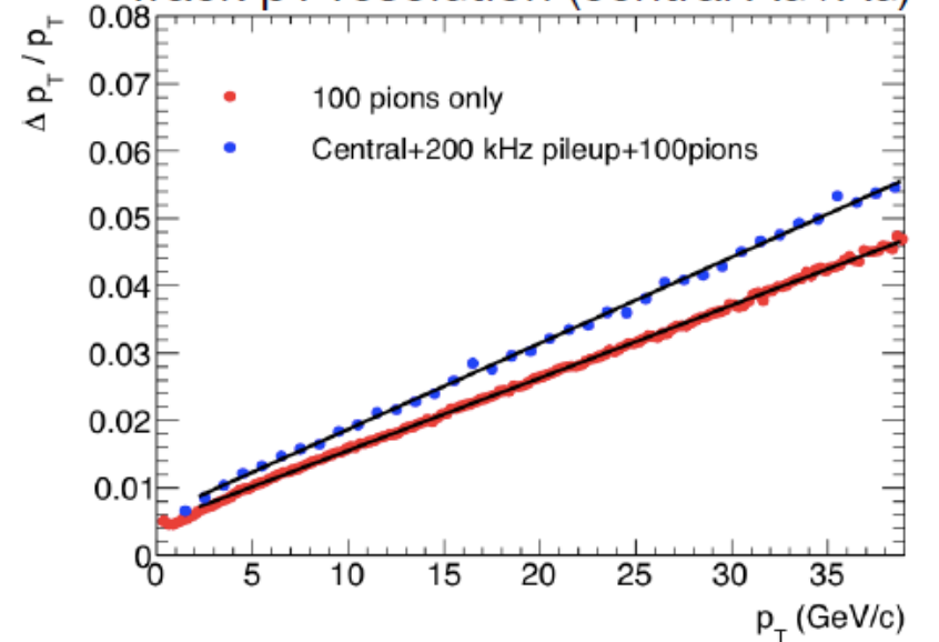
Track pT resolution (central Au+Au)
