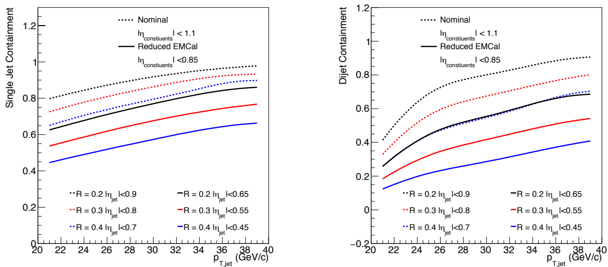
Figure 2.6: (Left) Fraction of inclusive single jets fully contained within the acceptance of the nominal ( |\eta| < 1.1 ) and reduced ( |\eta| < 0.85 ) EMCal configurations as a function of jet p_T and anti- k_T jet radius parameter. (Right) Fraction of dijets fully contained within the acceptance of the nominal ( |\eta| < 1.1 ) and reduced ( |\eta| < 0.85 ) EMCal configurations as a function of jet p_T and anti- k_T jet radius parameter.
