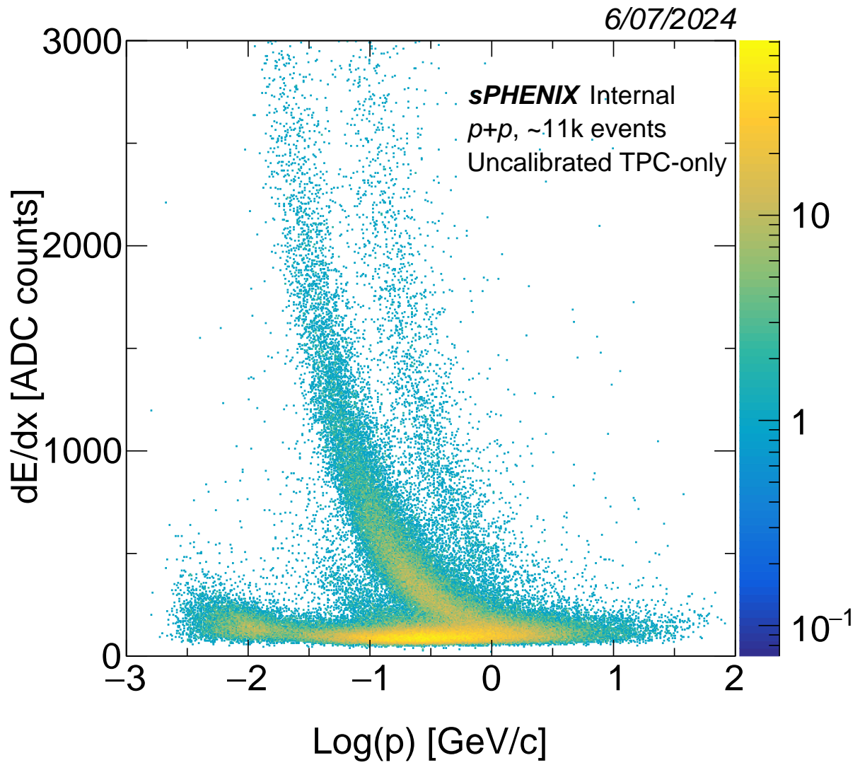
Figure 1: dE/dx
