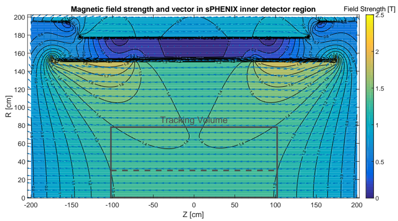
Figure 1.1: Magnetic field configuration in the tracking detector region.
