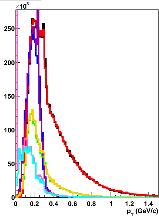
cluster p_T
