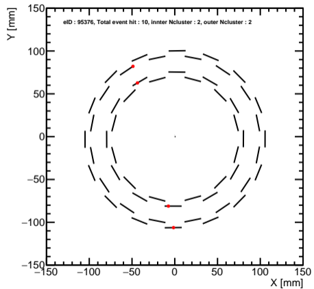
INTT event display X-Y plane
