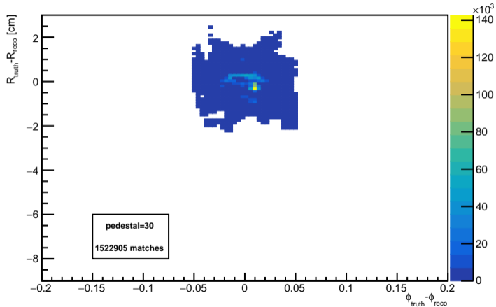
NN Method
