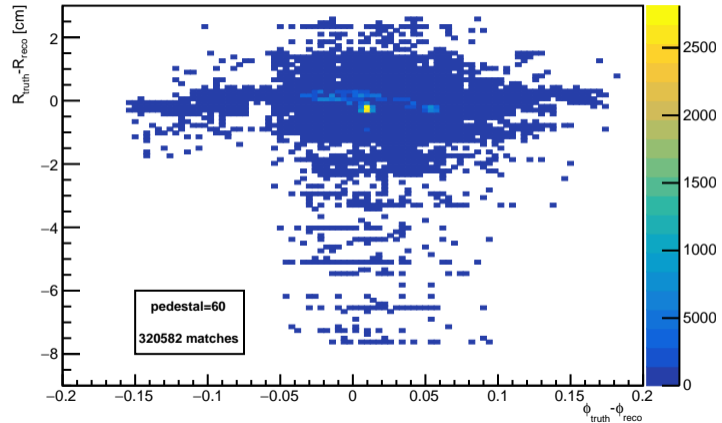
Fancy Method
