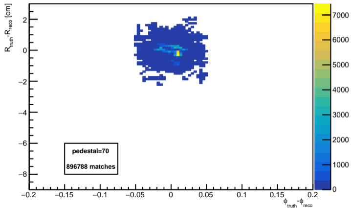
NN Method
