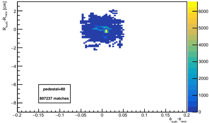
NN Method
