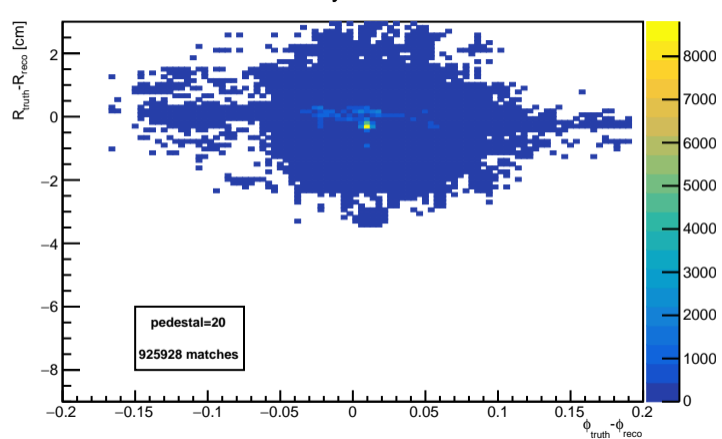
Fancy Method
