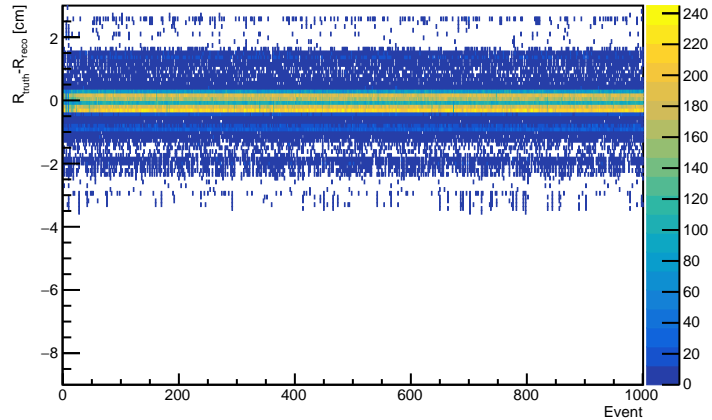
Fancy Method, pedestal=40
