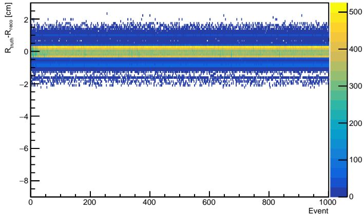
NN Method, pedestal=40
