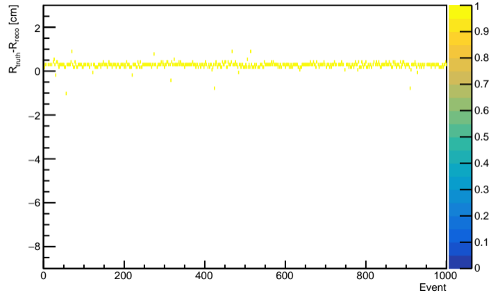
Fancy Method TruthIndex 1600, pedestal=20
