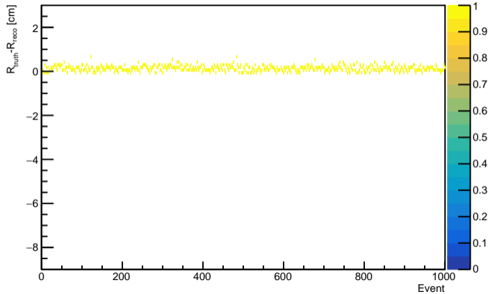
NN Method TruthIndex 1600, pedestal=80
