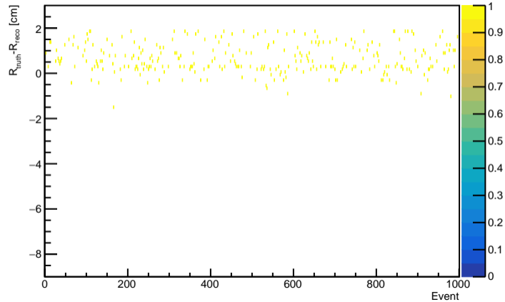
Fancy Method TruthIndex 1600, pedestal=0
