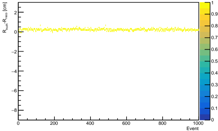
NN Method TruthIndex 1600, pedestal=50
