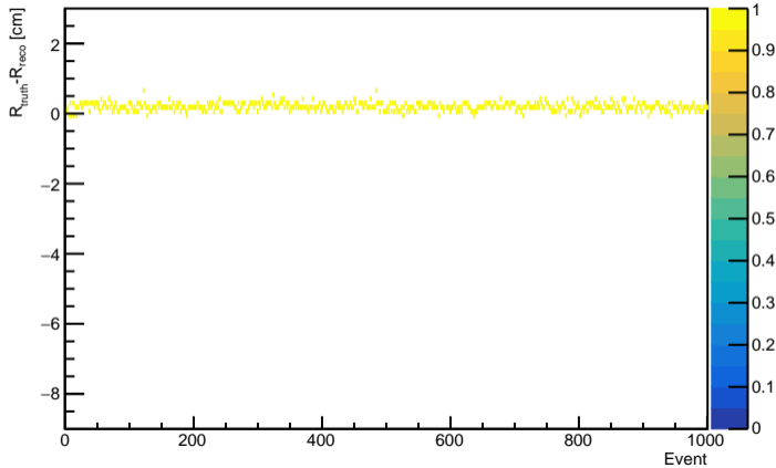
NN Method TruthIndex 1600, pedestal=60
