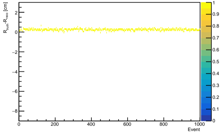
Fancy Method TruthIndex 1600, pedestal=40
