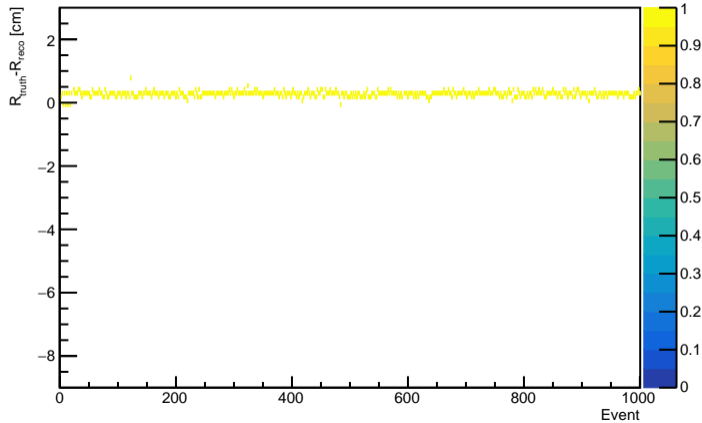
NN Method TruthIndex 1600, pedestal=20
