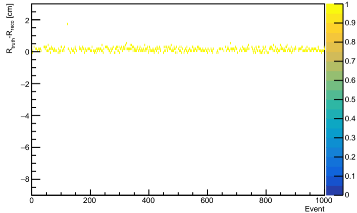
Fancy Method TruthIndex 1600, pedestal=80
