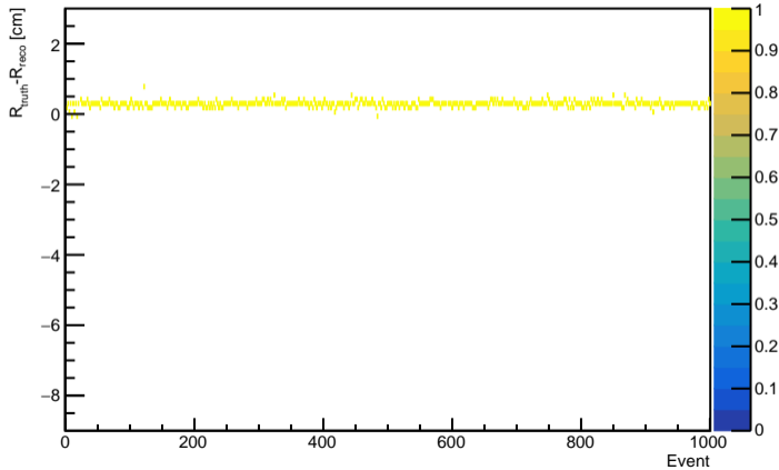
NN Method TruthIndex 1600, pedestal=10
