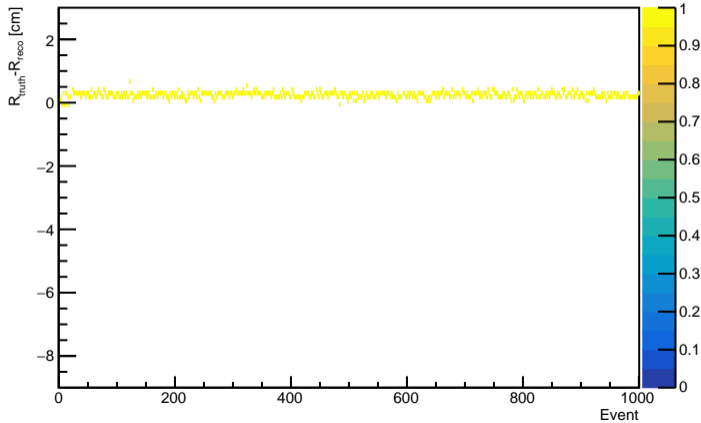
NN Method TruthIndex 1600, pedestal=40
