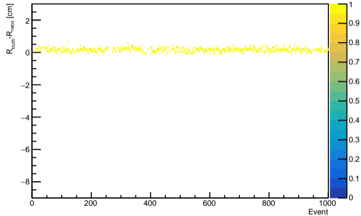
Fancy Method TruthIndex 1600, pedestal=70
