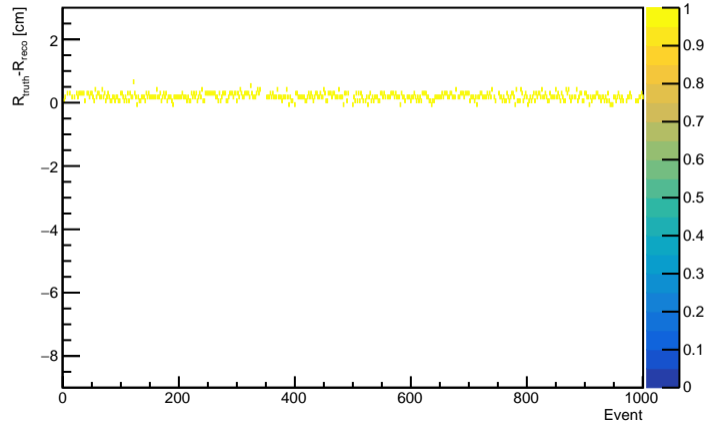
Fancy Method TruthIndex 1600, pedestal=60
