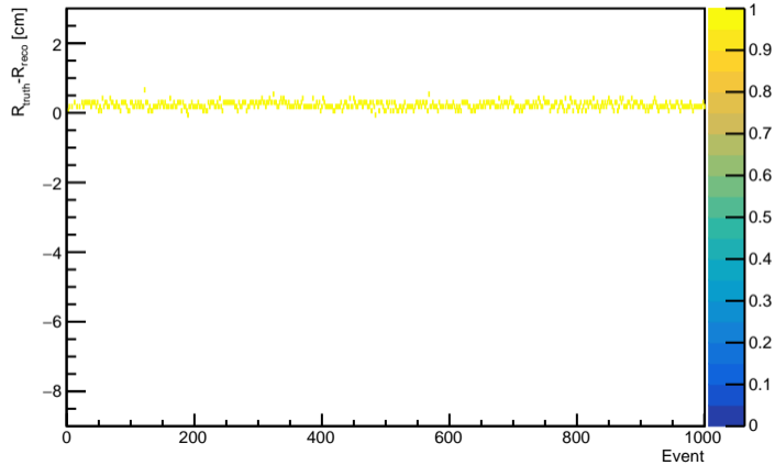
Fancy Method TruthIndex 1600, pedestal=50
