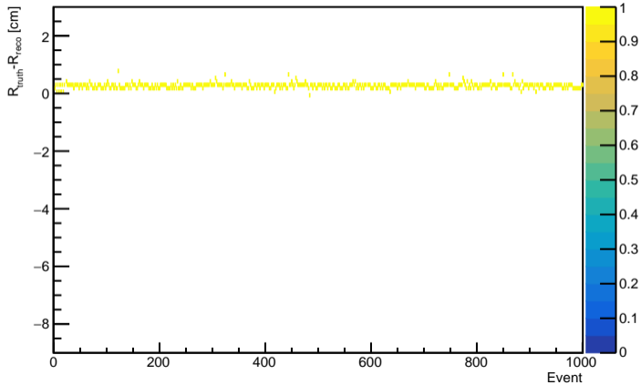
NN Method TruthIndex 1600, pedestal=0
