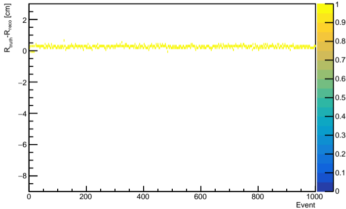
NN Method TruthIndex 1600, pedestal=30
