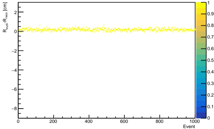
NN Method TruthIndex 1600, pedestal=70
