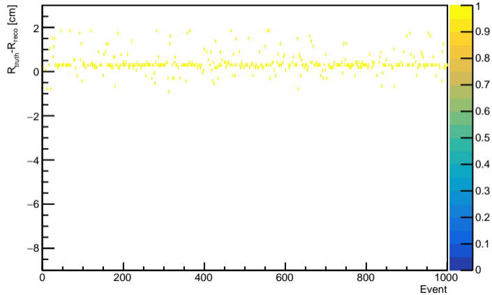
Fancy Method TruthIndex 1600, pedestal=10
