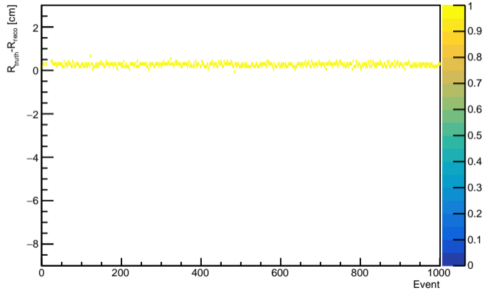
Fancy Method TruthIndex 1600, pedestal=30
