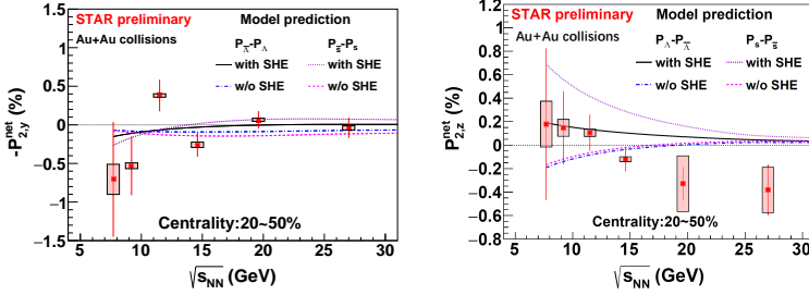
Figure 4: (Colour online) The net local polarization -P_{2,y}^{net} (left panel) and P_{2,z}^{net} (right panel) as a function of energy in Au+Au collisions. The red solid squares are data. Vertical lines and shaded boxes are statistical and systematic uncertainties.
