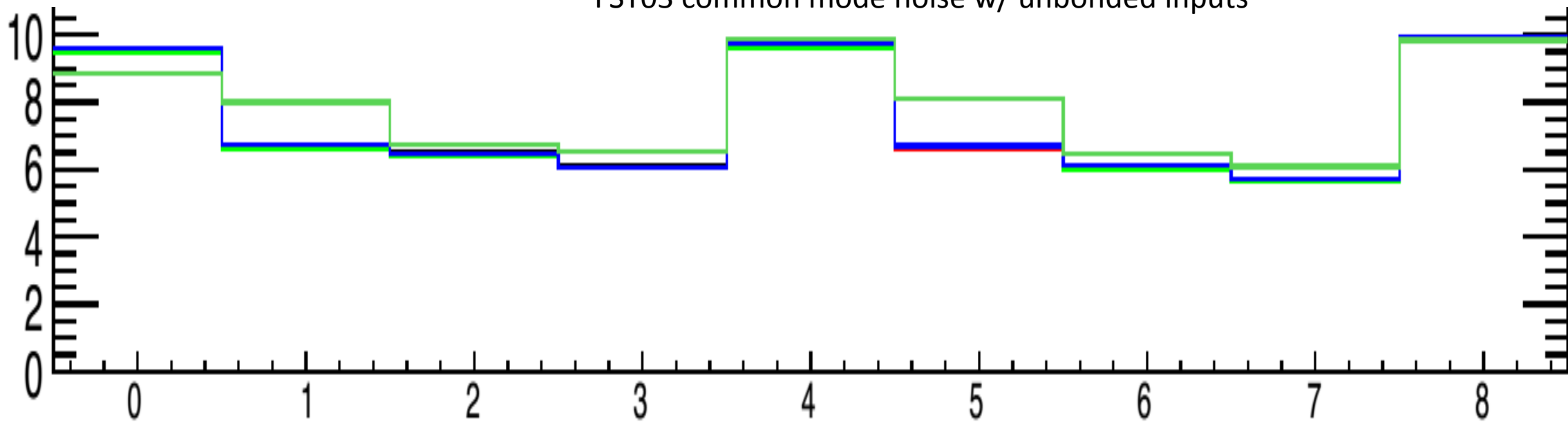
FST03 common mode noise w/ unbonded inputs
