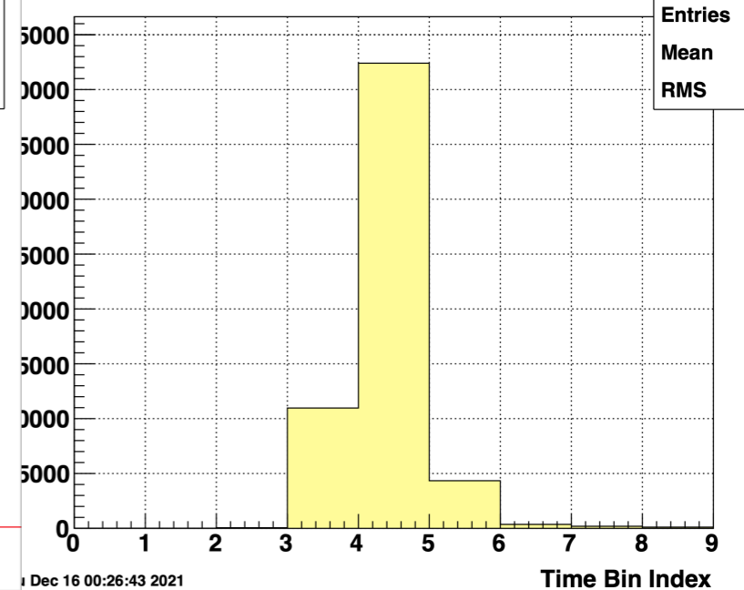
FST - Max ADC Time Bin (non-ZS)
