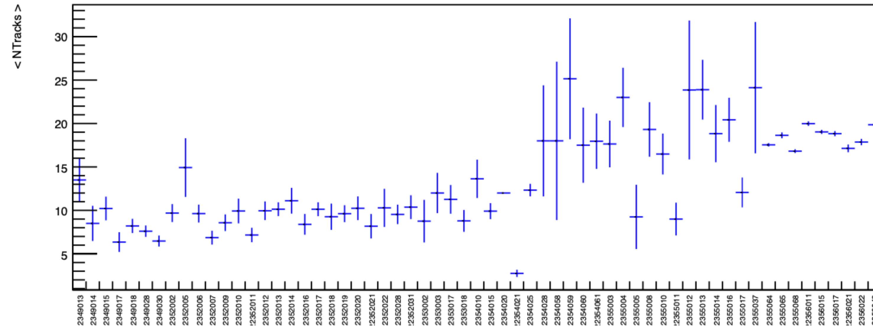
< NTracks > vs RunNumber - fcsJP2
