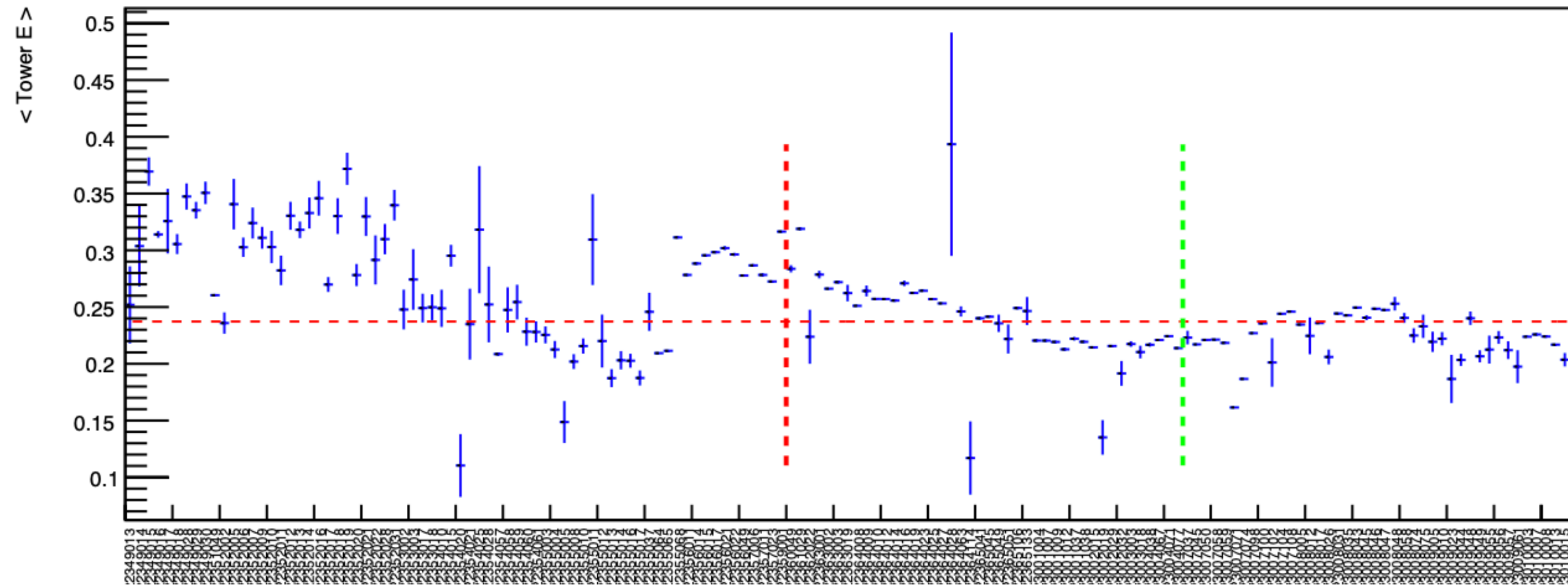
Ecal < Tower E > vs RunNumber - fcsJP2
