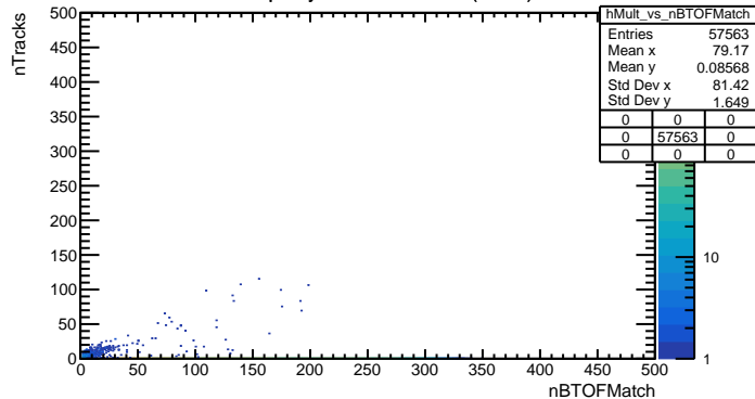
Multiplicity vs nBTOFMatch (Other)
