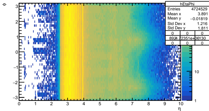
\eta vs \phi (Primary)
