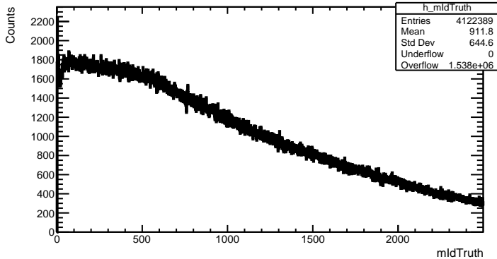
ID Truth (Global)
