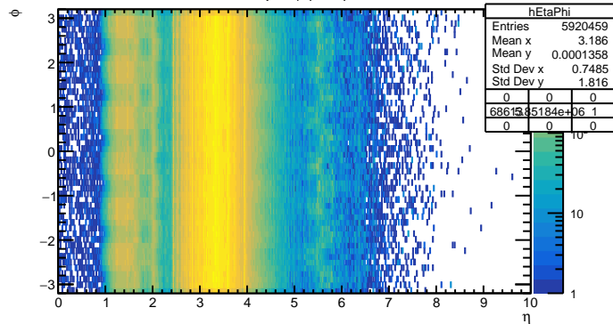
\eta vs \phi (BLC)
