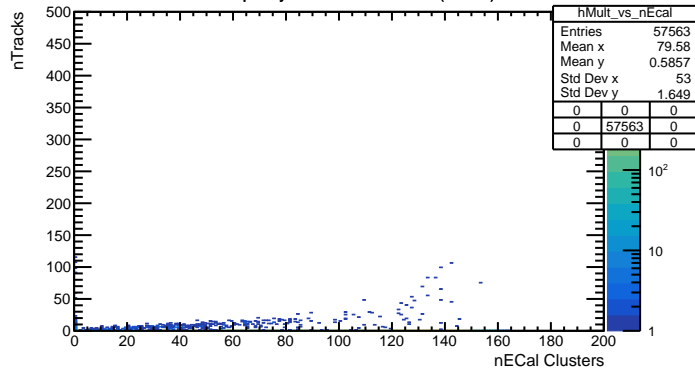
Multiplicity vs nEcal clusters (Other)
