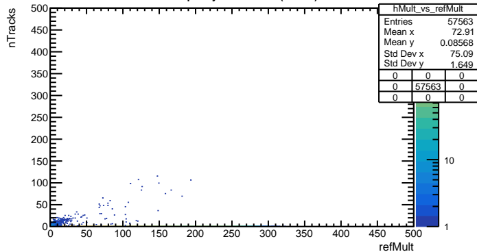
Multiplicity vs refMult (Other)
