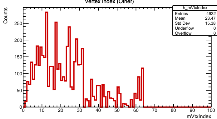
Vertex Index (Other)
