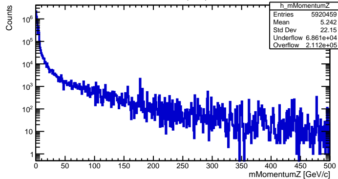
Momentum Z (BLC)
