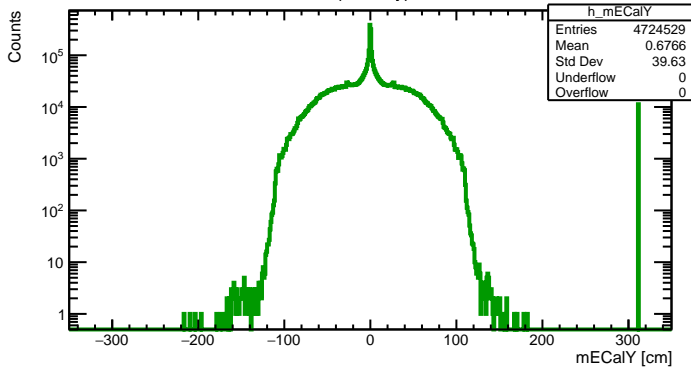
ECalY (Primary)
