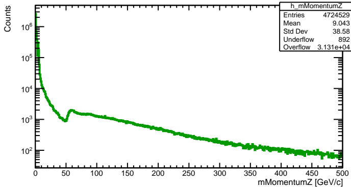
Momentum Z (Primary)
