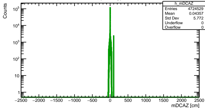
DCAZ (Primary)
