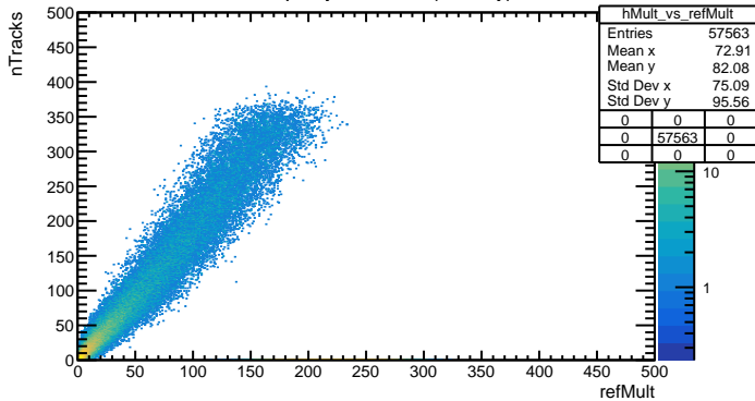
Multiplicity vs refMult (Primary)
