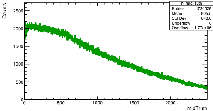
ID Truth (Primary)
