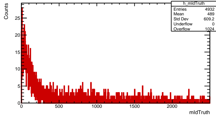
ID Truth (Other)
