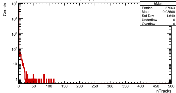
Multiplicity (Other)
