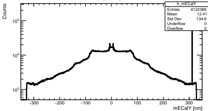
ECalY (Global)
