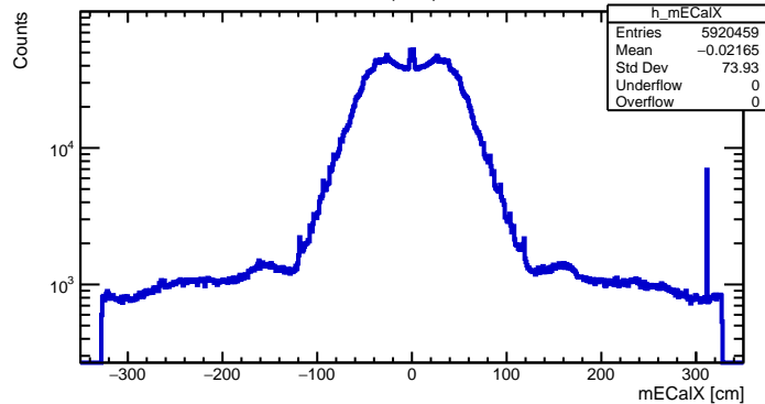
ECaIX (BLC)
