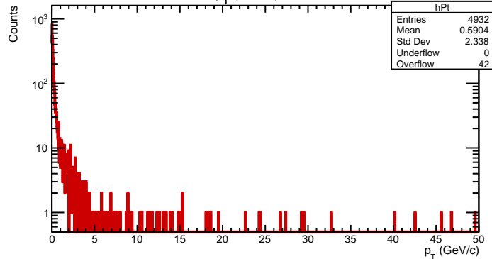
p_T (Other)
