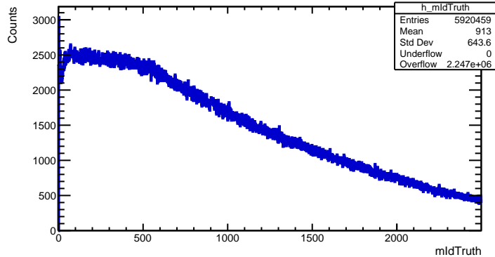
ID Truth (BLC)
