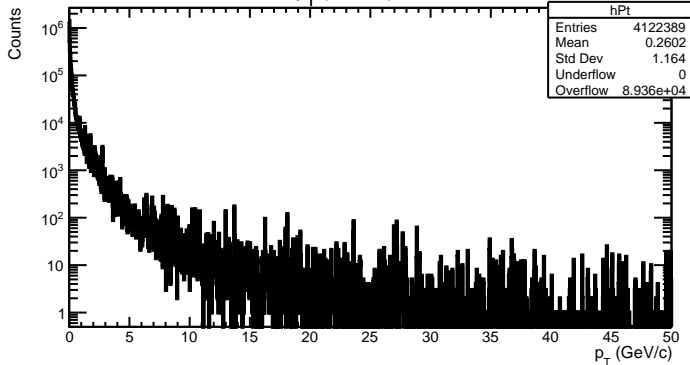
p_T (Global)
