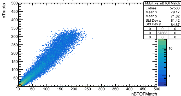
Multiplicity vs nBTOFMatch (Global)
