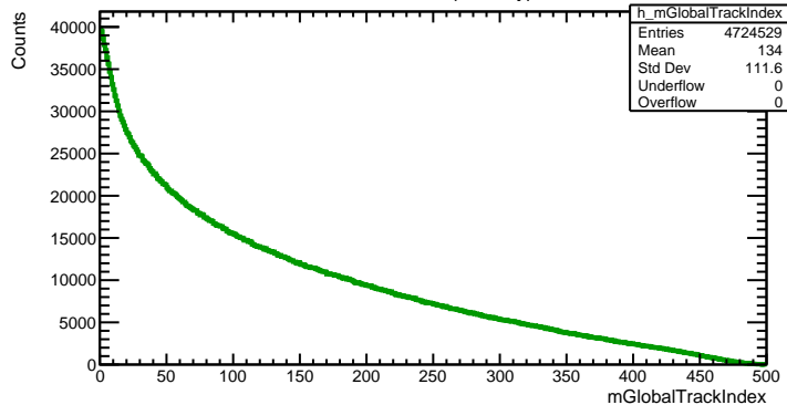
Global Track Index (Primary)
