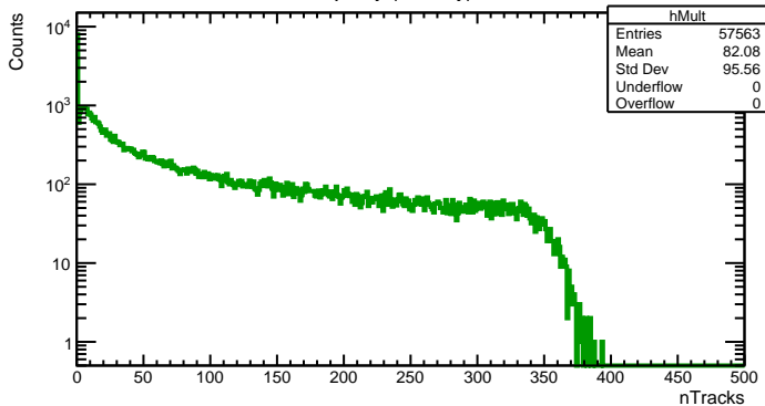
Multiplicity (Primary)
