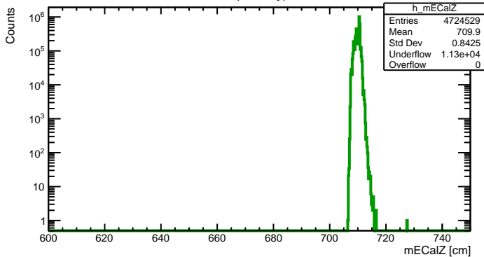
ECalZ (Primary)
