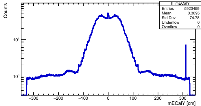
ECalY (BLC)
