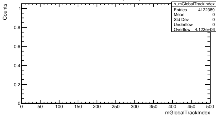
Global Track Index (Global)
