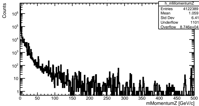
Momentum Z (Global)
