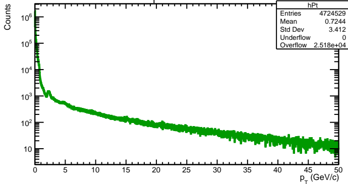
p_T (Primary)
