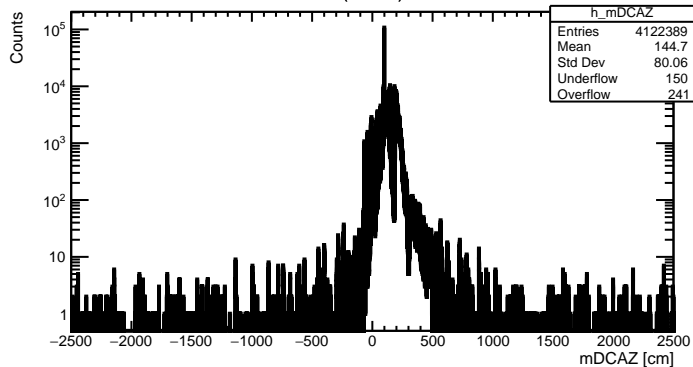
DCAZ (Global)
