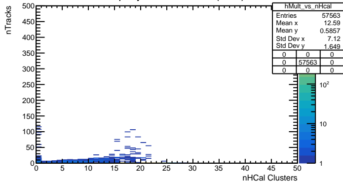
Multiplicity vs nHCal clusters (Other)
