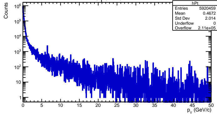
p_T (BLC)
