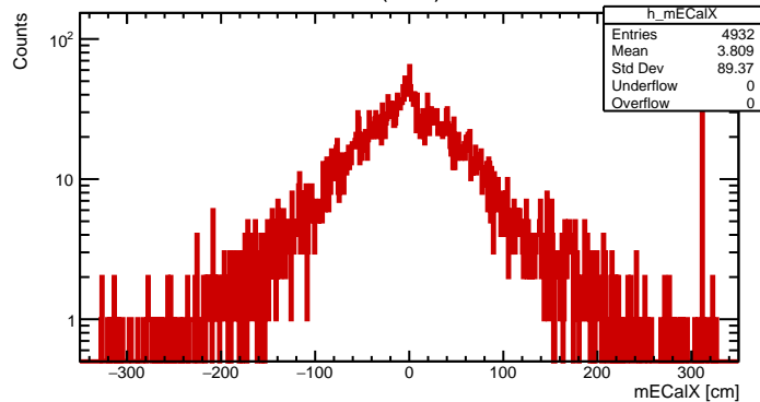
ECaIX (Other)
