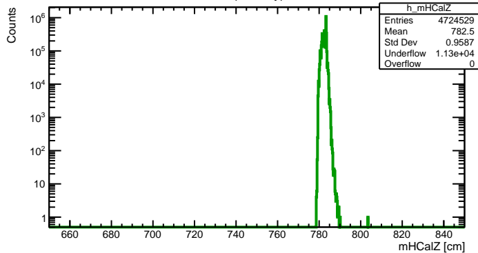
HCalZ (Primary)
