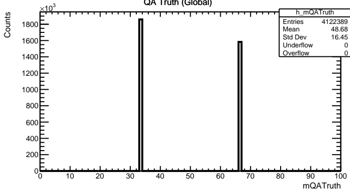
QA Truth (Global)
