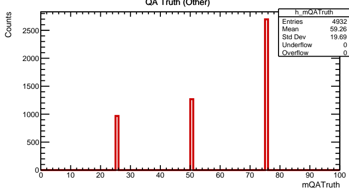
QA Truth (Other)
