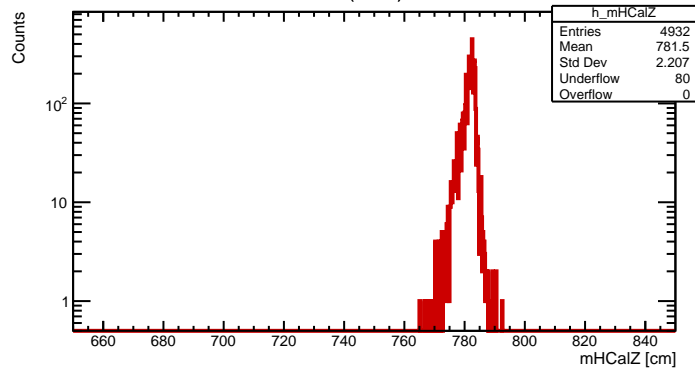
HCalZ (Other)
