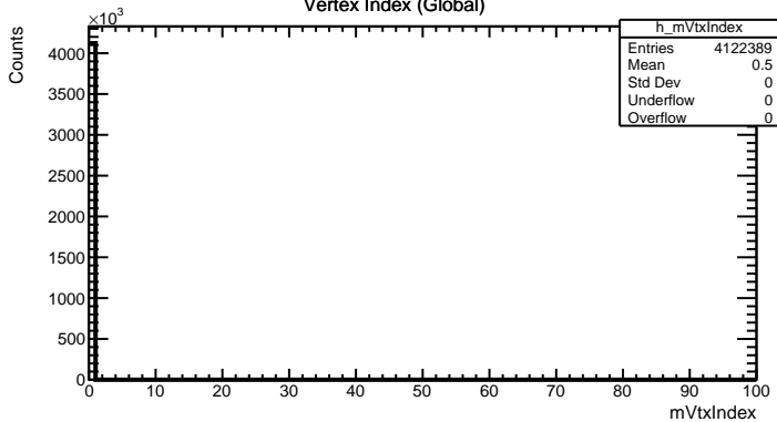
Vertex Index (Global)
