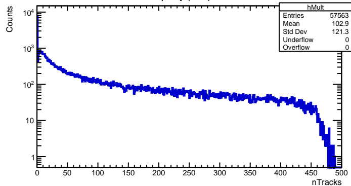
Multiplicity (BLC)
