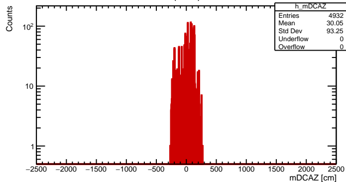
DCAZ (Other)
