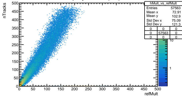
Multiplicity vs refMult (BLC)
