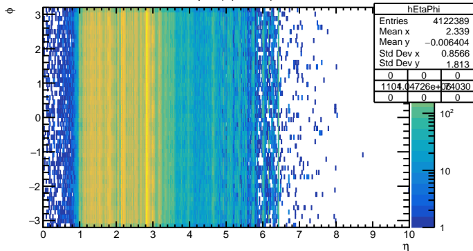
\eta vs \phi (Global)
