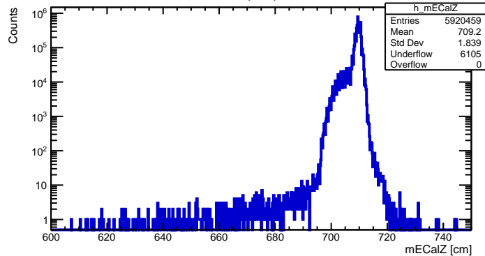
ECalZ (BLC)
