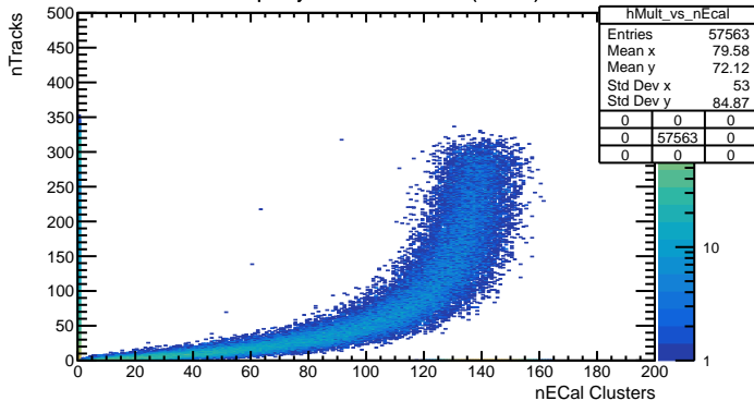
Multiplicity vs nEcal clusters (Global)
