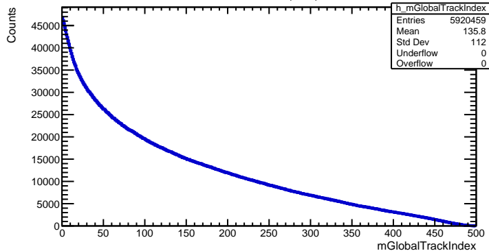
Global Track Index (BLC)
