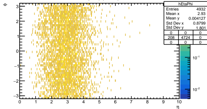
\eta vs \phi (Other)
