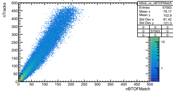
Multiplicity vs nBTOFMatch (BLC)
