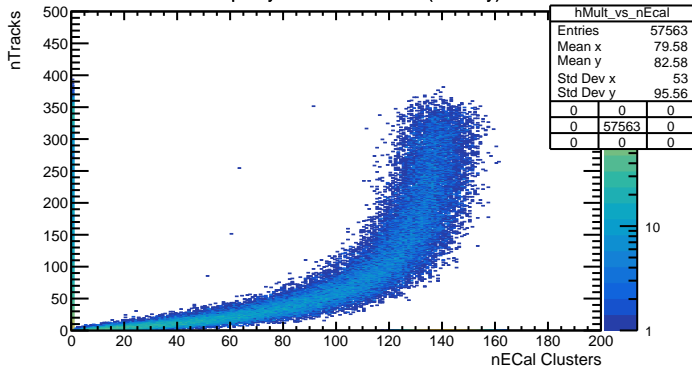
Multiplicity vs nEcal clusters (Primary)
