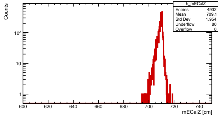
ECalZ (Other)
