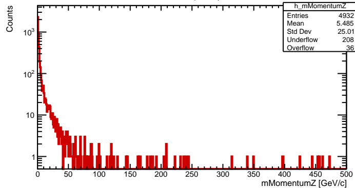
Momentum Z (Other)
