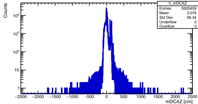
DCAZ (BLC)
