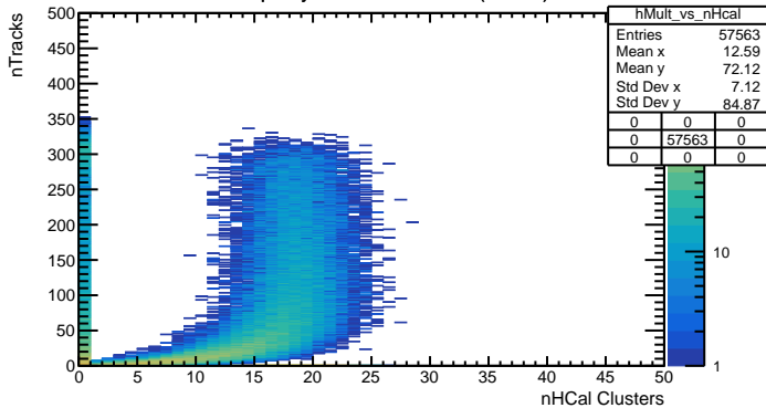
Multiplicity vs nHCal clusters (Global)
