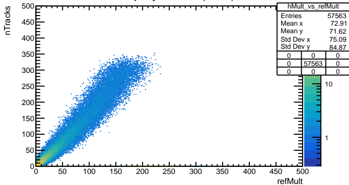
Multiplicity vs refMult (Global)
