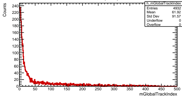
Global Track Index (Other)
