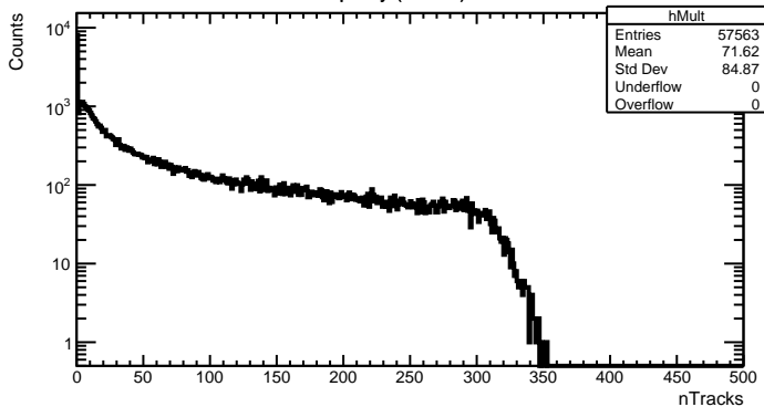
Multiplicity (Global)
