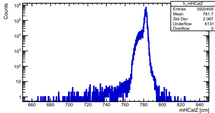
HCalZ (BLC)
