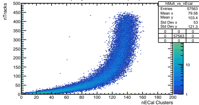
Multiplicity vs nEcal clusters (BLC)
