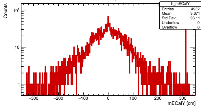
ECalY (Other)
