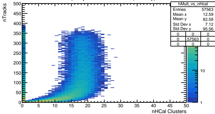
Multiplicity vs nHCal clusters (Primary)
