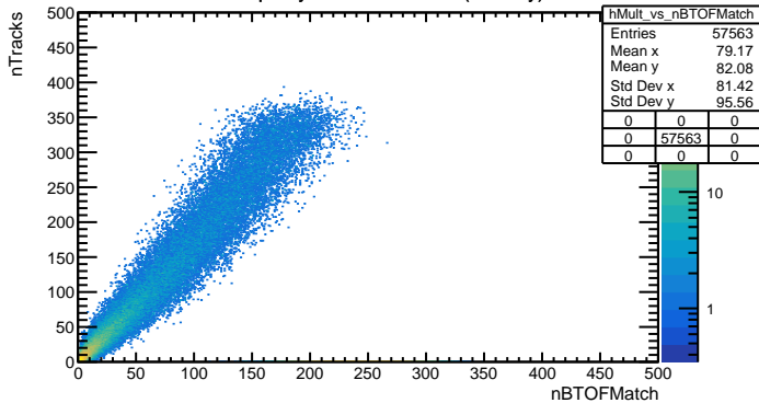
Multiplicity vs nBTOFMatch (Primary)
