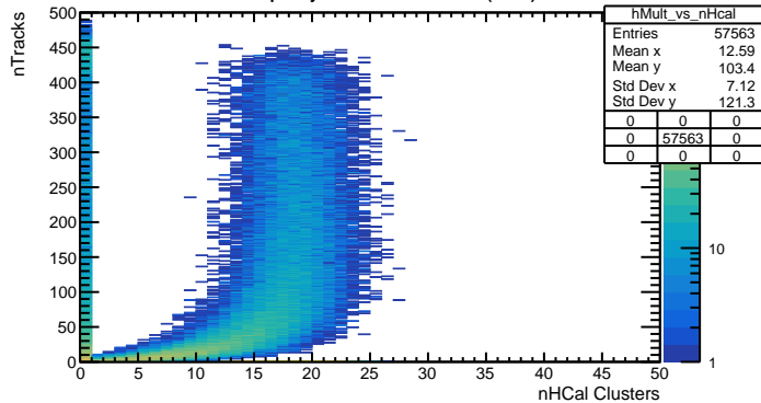
Multiplicity vs nHCal clusters (BLC)
