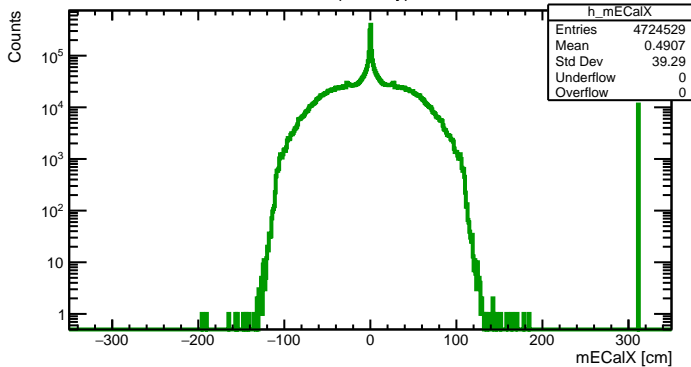
ECaIX (Primary)
