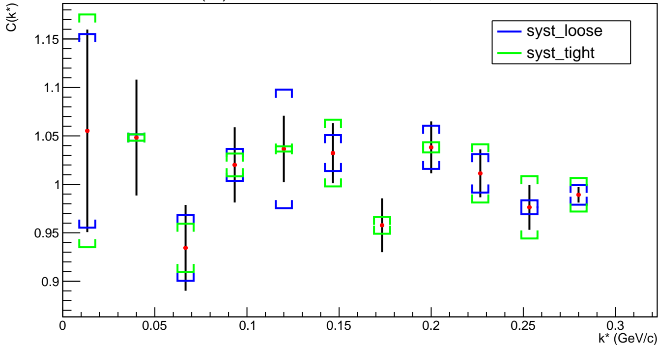
C(k*) distribution for D0-Kaon, Au+Au@2014
