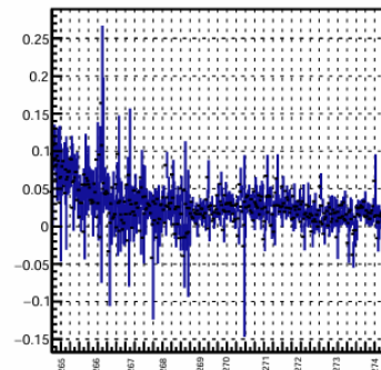
Average full jet phi
