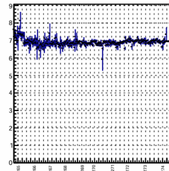
Average full jet pt
