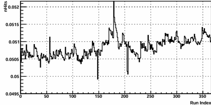
EMC hit > 1 GeV
