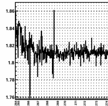
Dev charged jets phi
