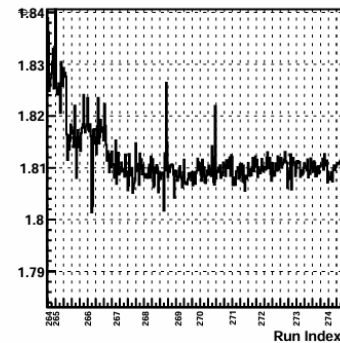
Dev track phi
