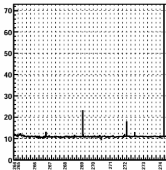
Dev full jets pt
