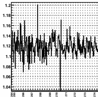
Dev #full jets
