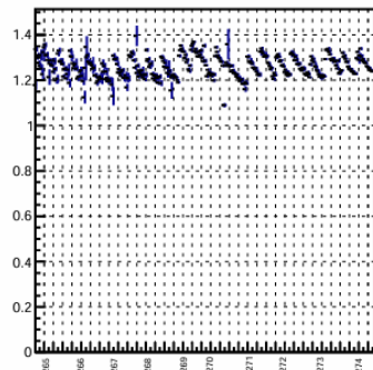
Average number of full jet
