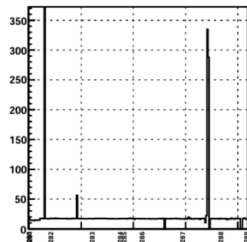
Dev full jets pt
