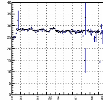
Average full jet pt
