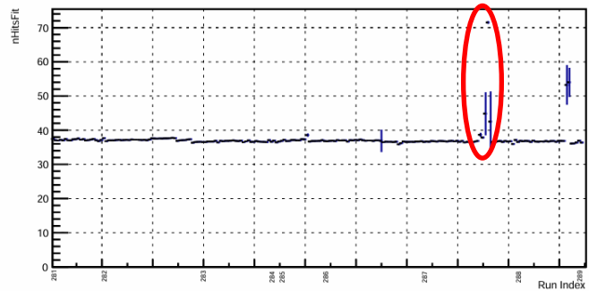
Dev track nhit
