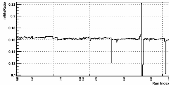
Dev track nhitratio
