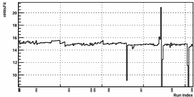
Dev track nhit
