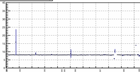
Average full jet bkg. sub. p_T
