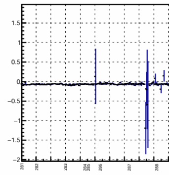
Dev charged jets phi
