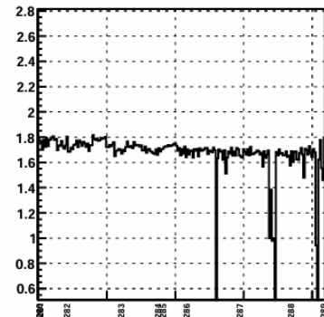
Dev #full jets
