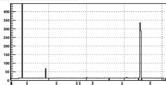
Dev Background Subtracted full jets pt
