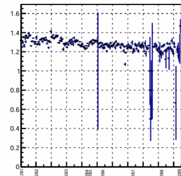
Average number of full jet
